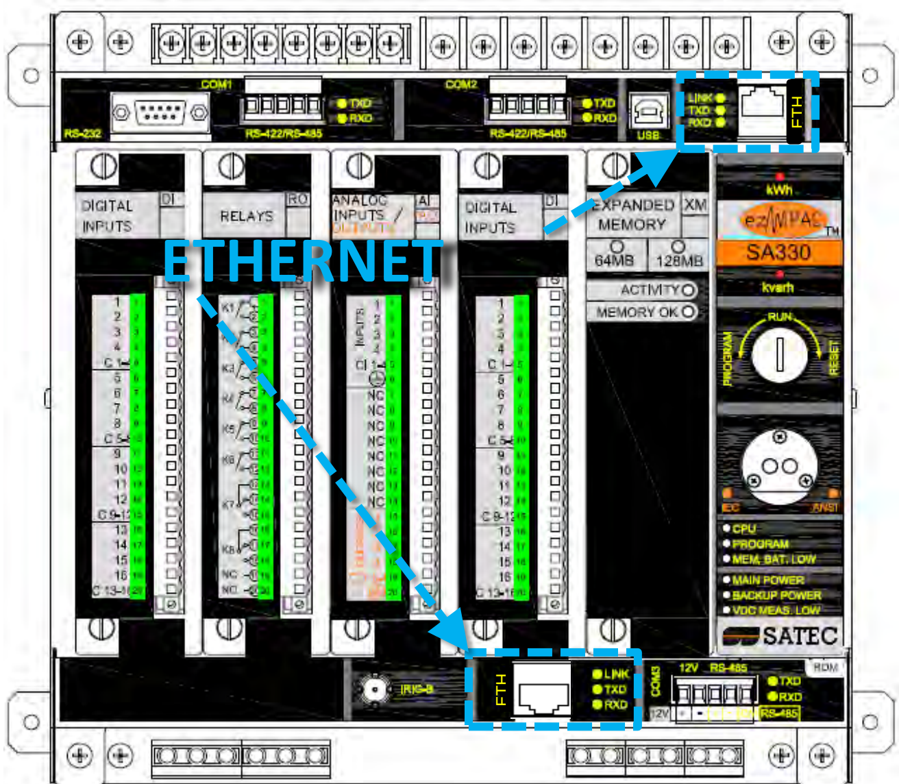
Figure 1: Dual Ethernet Port ezPAC top view.
