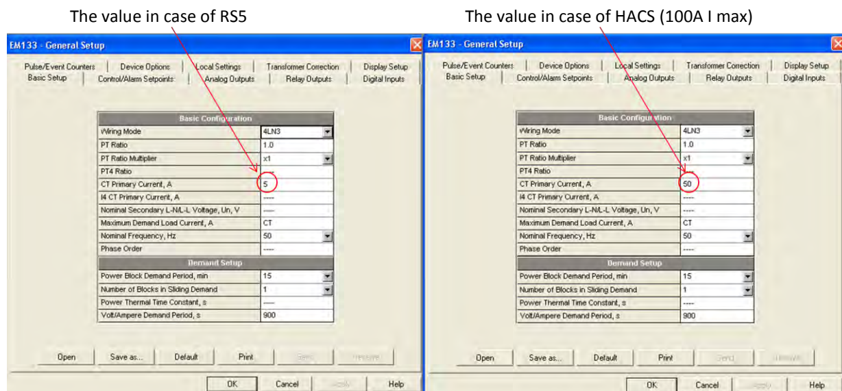
Figure 3: In device General Setup (PAS Software) "CT Primary Current" should be modified with the nominal value of the used CT (the illustrated cases are RS5 (In=5A) and HACS for 100A (In=50A)).
