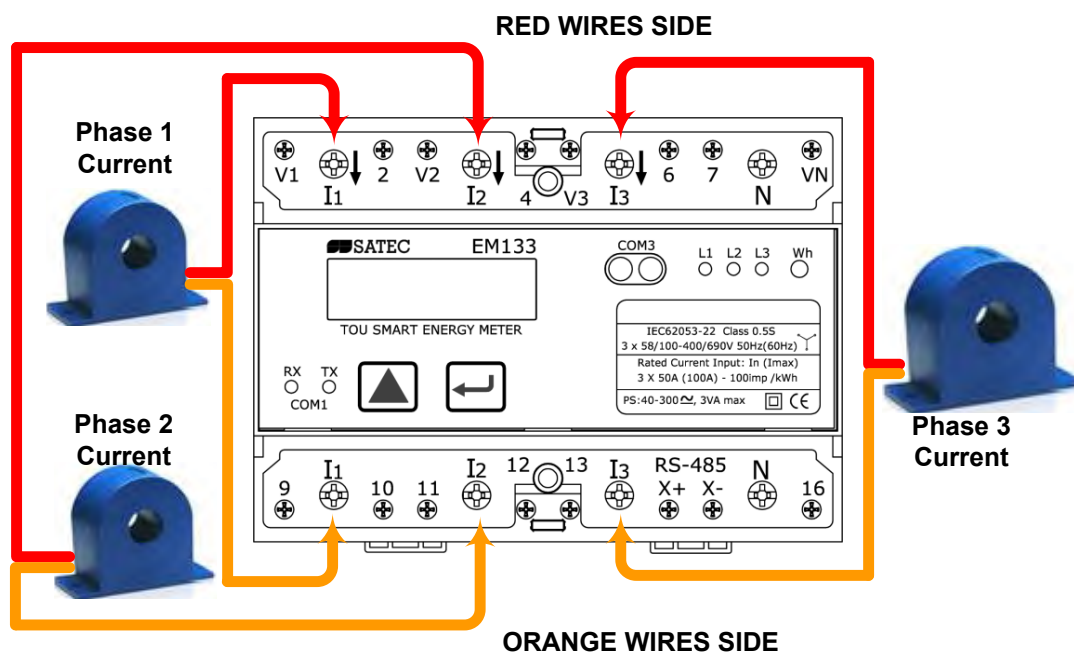
Figure 2: HACS Solid CT connection
